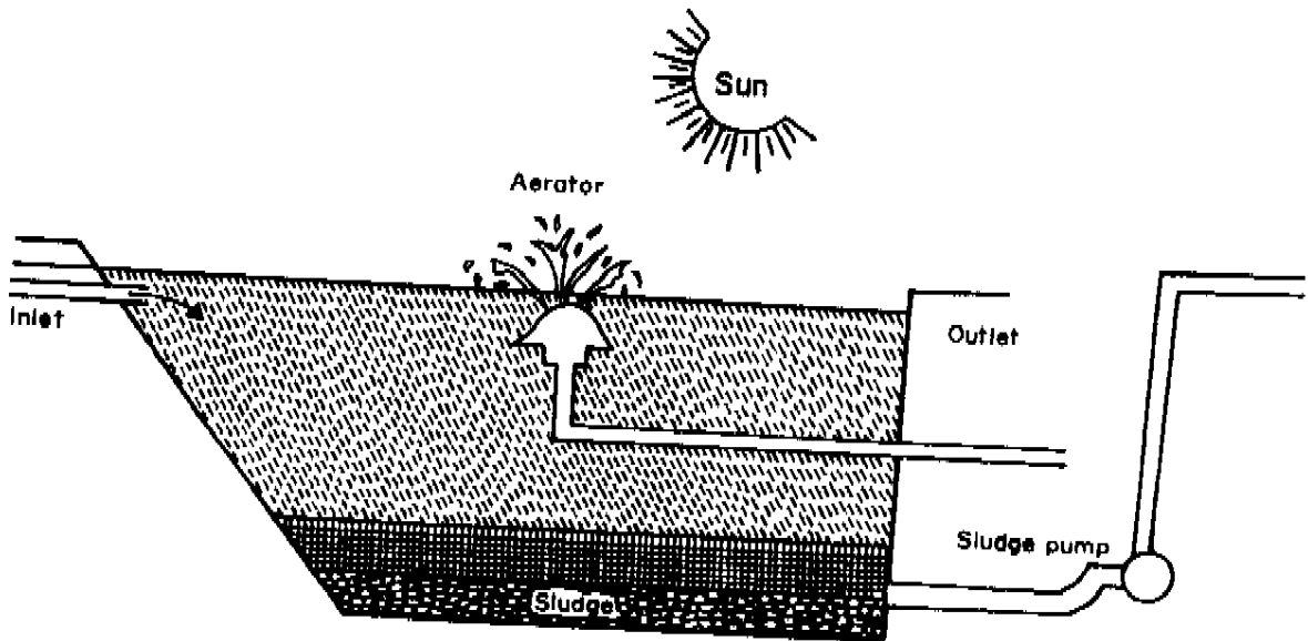
Figure 2. Aeration tank
